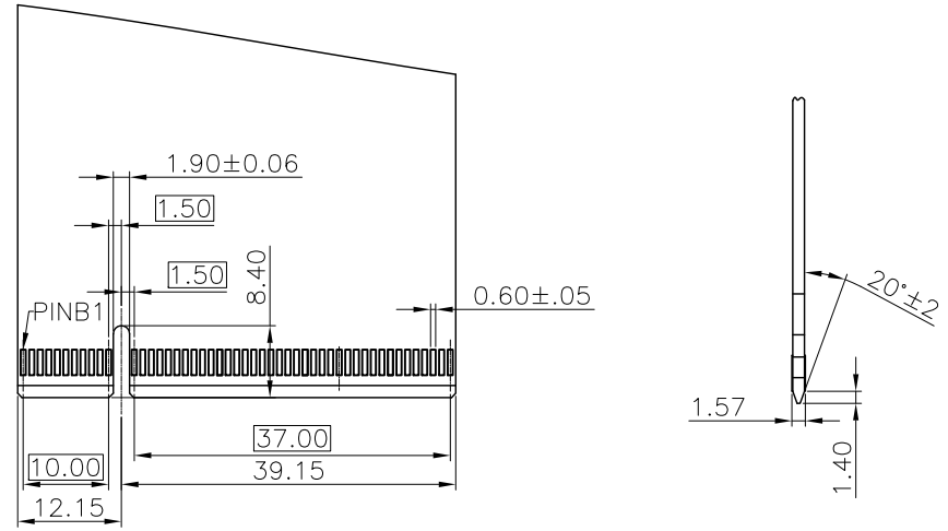
PRIMARY (COMPONENT) SIDE
