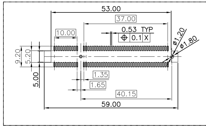
RECOMMENDED PCB LAYOUT DEFAULT TOLERANCE ±0.05
